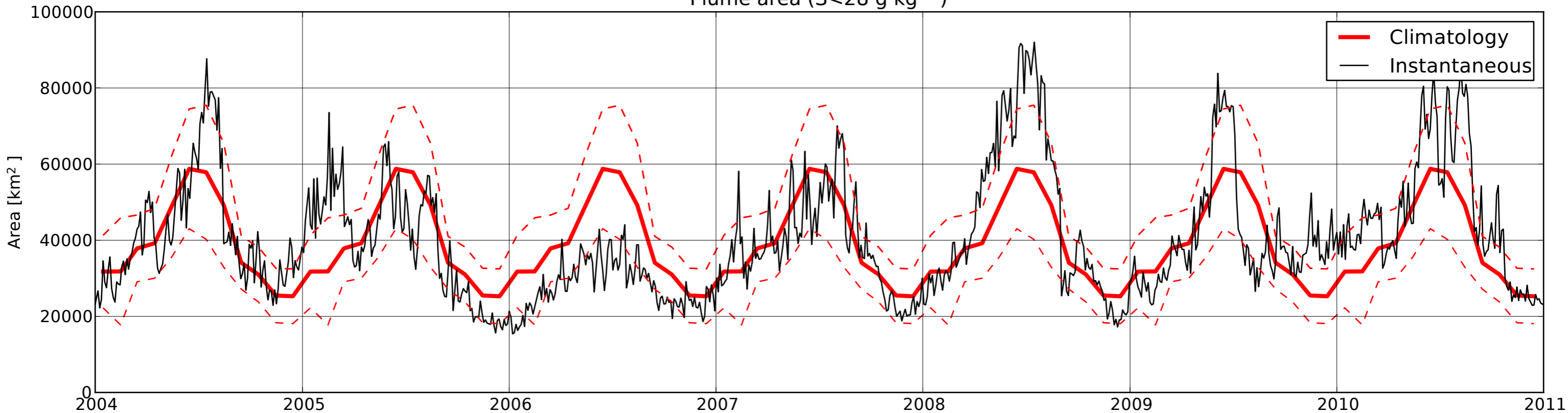
Plume area ( S < 28 \text{ g kg}^{-1} )
